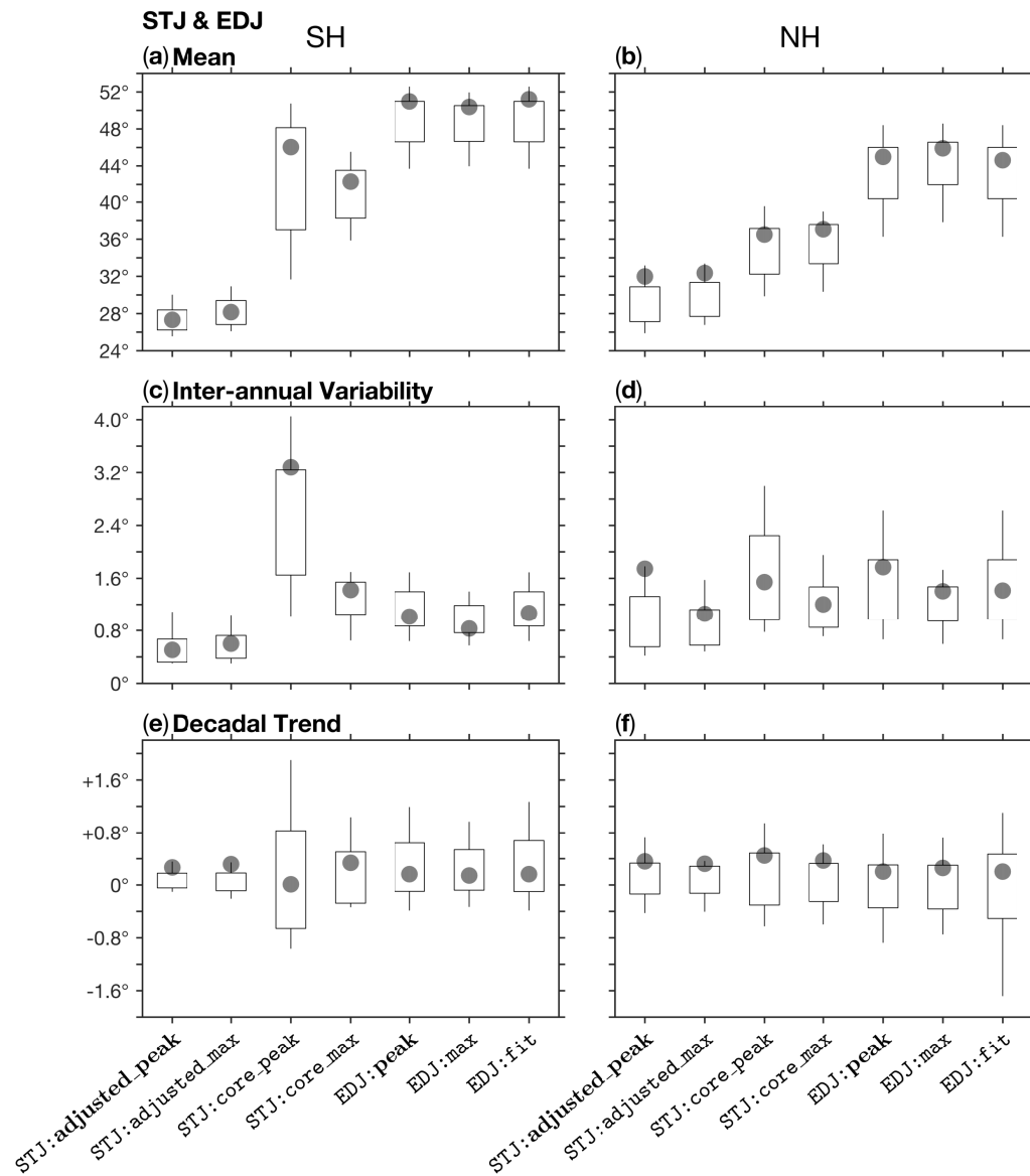
Figure S8. As in Fig. S5 for the STJ and EDJ metrics.
