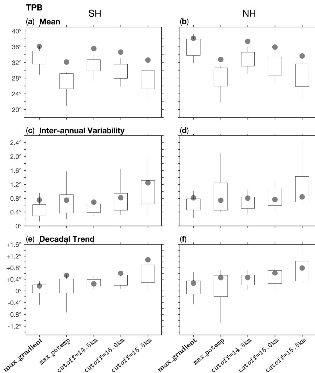
Figure S6. As in Fig. S5 for the TPB metric. For the cutoff method, geopotential height cutoff values of 14500m, 15000m (default), and 15500m are shown. (For Cutoff=15,500 and for max_potemp , three of the models produced unrealistic results and were removed from the analysis).
