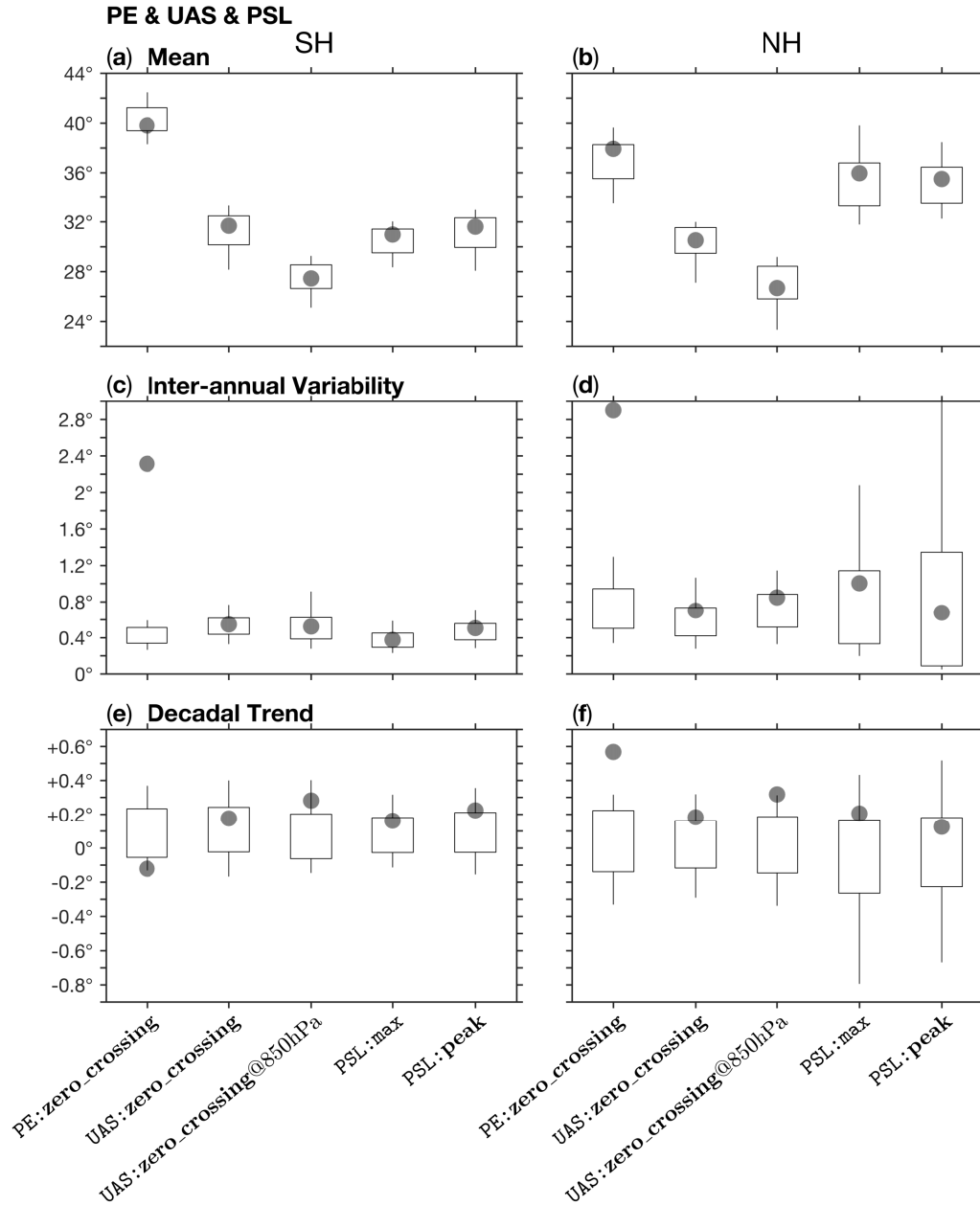
Figure S9. As in Fig. S5 for the PE, UAS, and PSL metrics. For UAS, the default and only method, zero_crossing , is shown for both the surface wind and the zonal-mean wind at the 850 hPa level. The input parameter Lat_Uncertainty is set to zero (default) in all of the methods.
