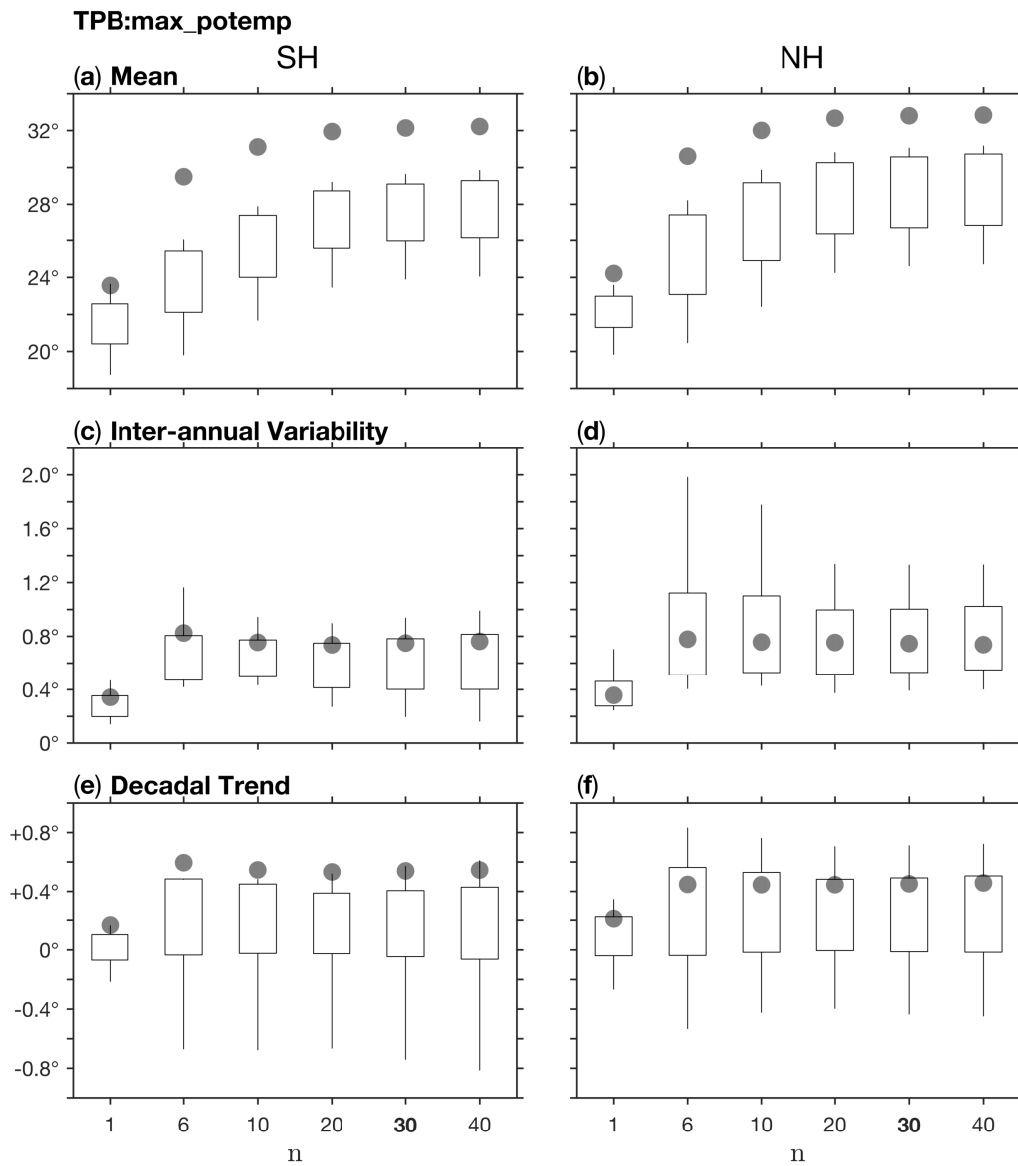
Figure S4. As in Fig. S1 for the dependence of TPB:max_potemp on the smoothing parameter n .
