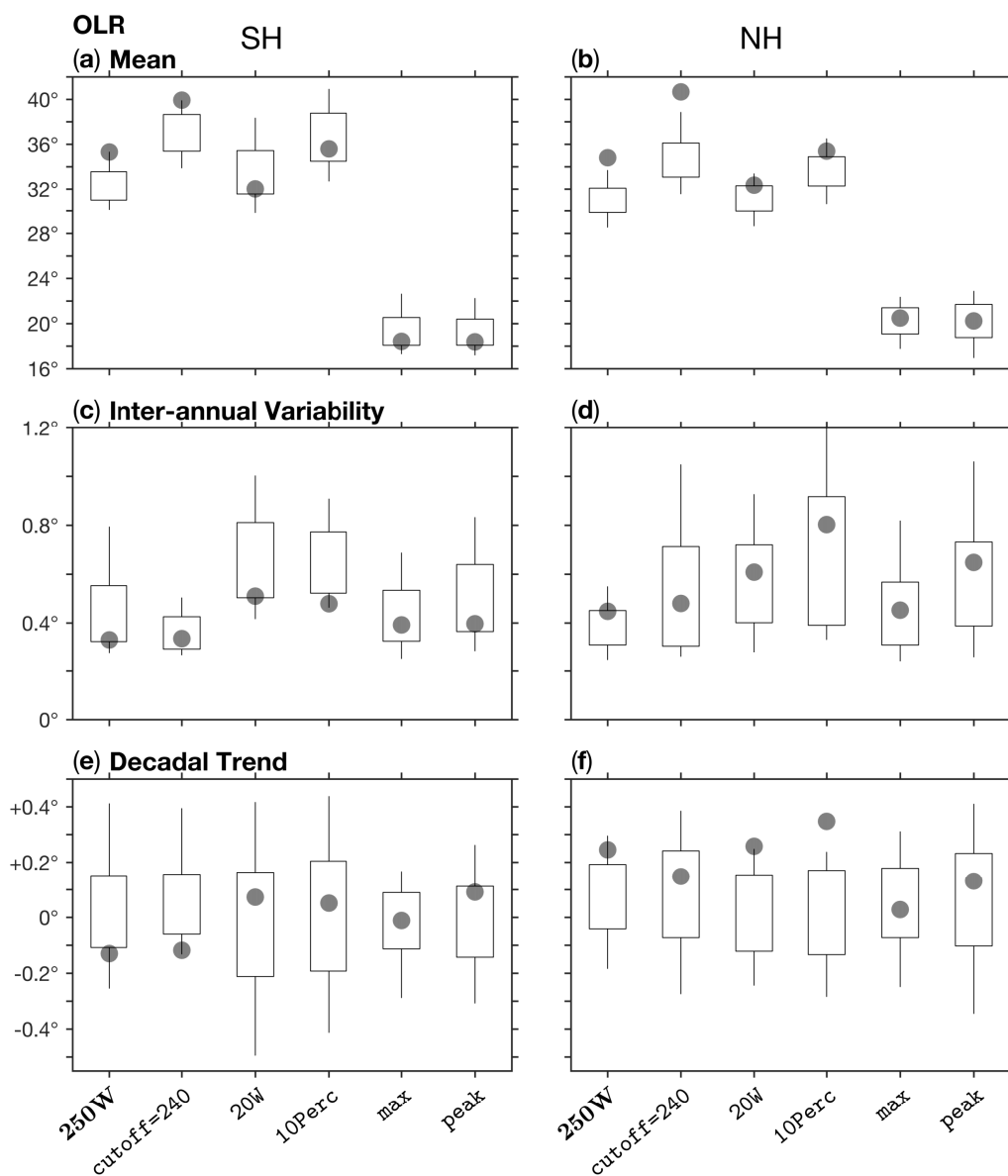
Figure S7. As in Fig. S5 for the OLR metric. The cutoff method is shown for the cutoff parameter Cutoff=240 Wm -2 .
