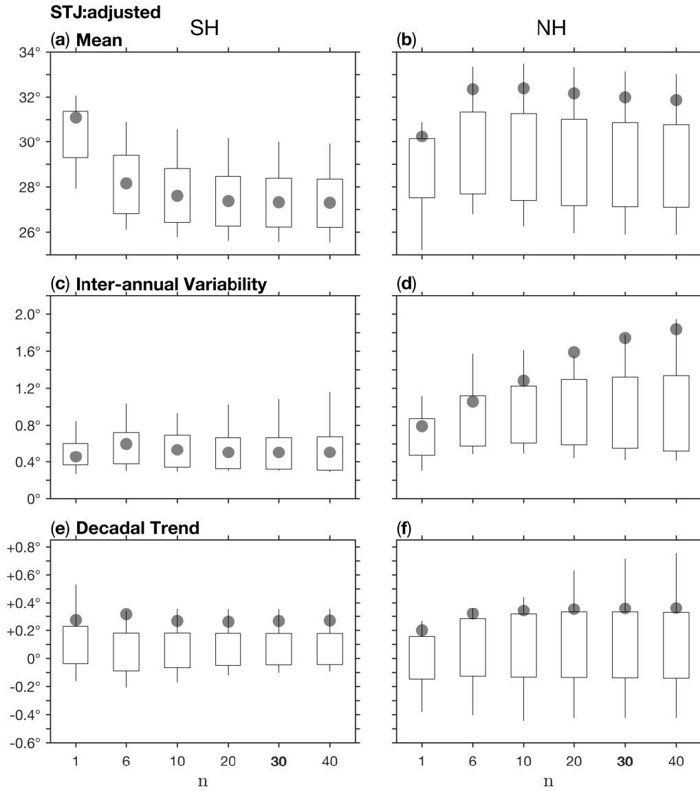
Figure S2. As in Fig. S1 for the dependence of STJ:adjusted on the smoothing parameter n .
