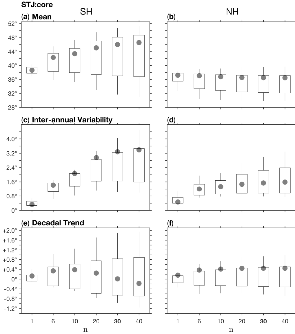
Figure S1. The dependence of the mean latitude (first row), inter-annual variability (second row), and trend ( ^{\circ} /decade, third row) on the smoothing parameter n for the STJ:core method, derived from annual means of the zonal-mean zonal wind in the SH (left column) and NH (right column), for the period 1979–2004. The default value of n (30) is bolded. For simplicity, positive values are used for both the NH and SH. Candle boxes show mean \pm 1 standard deviation of CMIP5 inter-model spread. Candle wicks show maximal and minimal CMIP5 model values. ERAI values are shown in gray dots.
