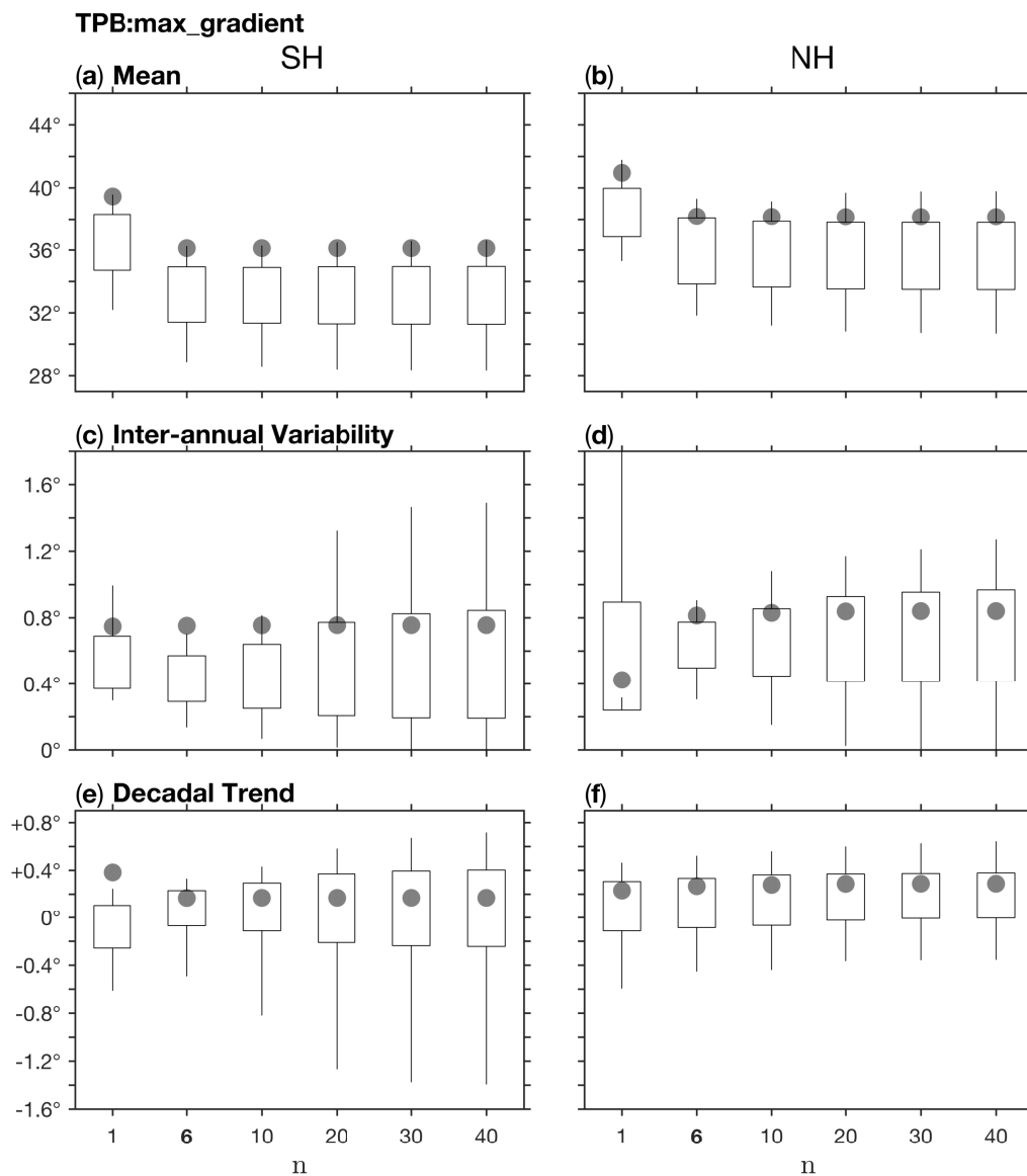
Figure S3. As in Fig. S1 for the dependence of TPB:max\_gradient on the smoothing parameter n .
