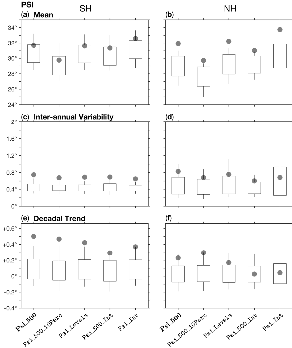
Figure S5. The mean latitude (first row), inter-annual variability (second row), and trend ( ^{\circ} /decade, third row) of the 5 available PSI metric methods, derived from annual means of the zonal-mean meridional wind in the SH (left column) and NH (right column), for the period 1979–2004. The default method ( Psi_500 ) is bolded. For simplicity, positive values are used for both the NH and SH. Candle boxes show mean \pm 1 standard deviation of CMIP5 inter-model spread. Candle wicks show maximal and minimal CMIP5 model values. ERAI values are shown in gray dots. The input parameter Lat_Uncertainty is set to zero (default) in all of the methods.
